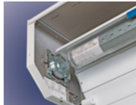
Safety Brake
