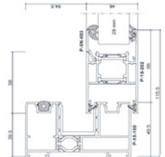
Threshold and Sash
