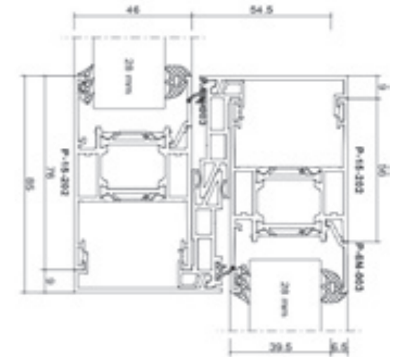
Standard Interlock
